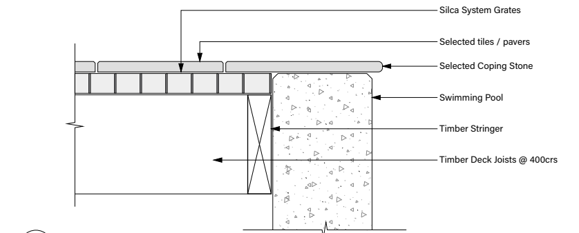
Silca System on timber deck joists - Pool Edge
