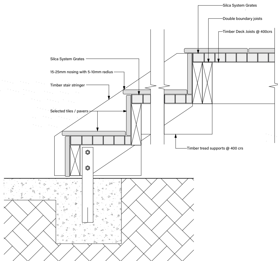
Silca System on timber steps (private or common stairway)
