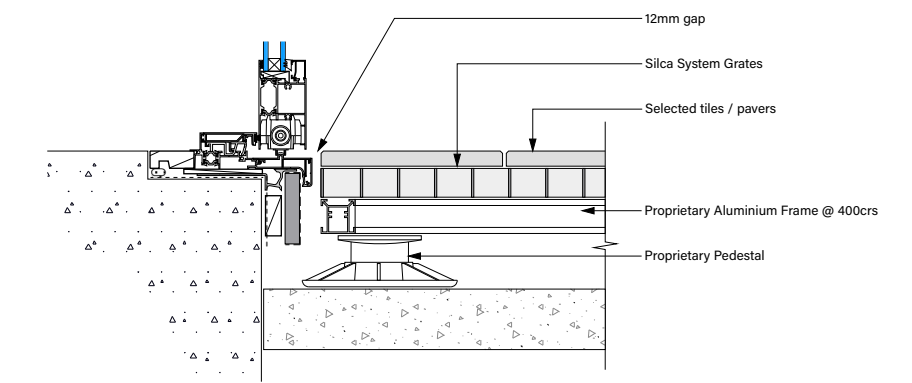
Silca System on aluminium frame and pedestals
