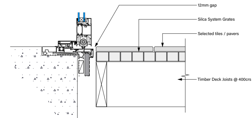
Silca System on timber deck joists at door threshold
