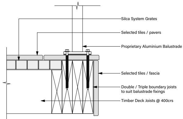
Silca System on timber deck joists - Top Mount Balustrade
