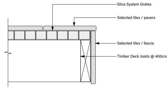
Silca System on timber deck joists - Fascia Edge
