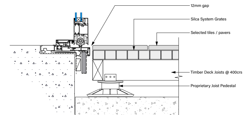
Silca System on timber deck joists and joist pedestals
