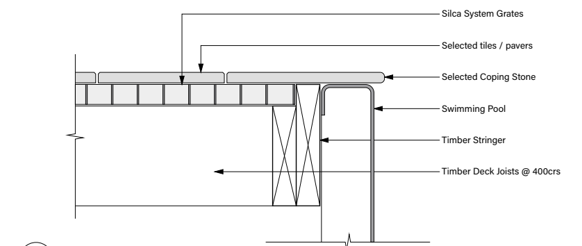
Silca System on timber deck joists - Pool Edge
